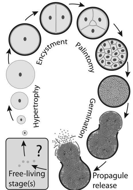
Fig. 4. Proposed life cycle of Tianzhushania through hypertrophic growth of mother cell, encystment in multilayered wall, palintomic cleavage resulting in a tightly packed mass of pre-propagules, germination by opening of outer cyst wall, and release of propagules by degradation of inner cyst wall. Shown is the role of the outer and inner cyst walls in forming the peanut-shaped germination stages (see also modern mesomycetozoean examples in fig. S7). The outer cyst wall (seldom preserved) is indicated in black; the inner cyst wall dark is indicated in gray.
