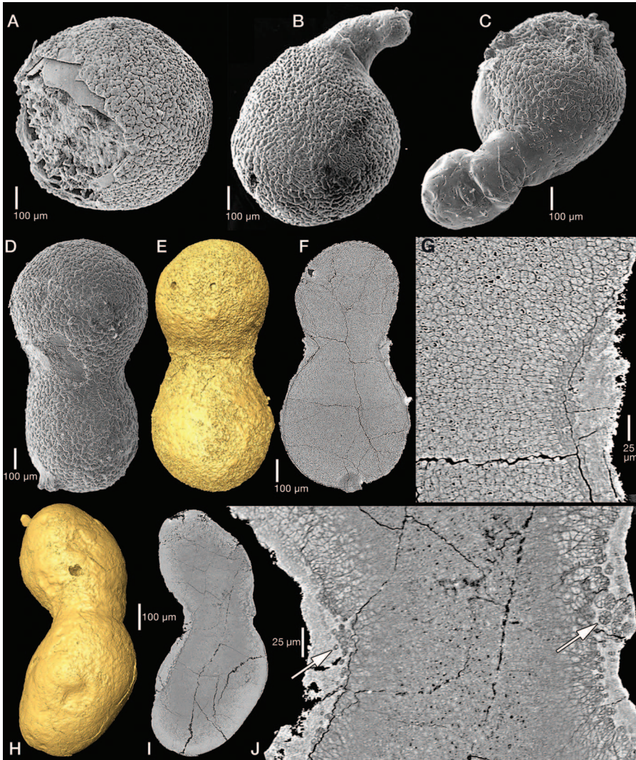
Fig. 3. Tianzhushania from the Ediacaran Doushantuo Formation, Datang Quarry, Weng’an, Guizhou Province, China. (A) Regular and (B to J) irregular forms, the latter interpreted to be in the germinating stage: MESIG 10022 [(A) SEM micrograph]; MESIG 10023 [(B) SEM micrograph (19)]; MESIG 10024 [(C) SEM micrograph (19)]; MESIG 10021 [(D) SEM micrograph]; SMNH X 4447 [(E) to (G) srXTM renderings]; SMNH X 4448 [(H) to (J) srXTM renderings]. (A) Surface of regular globular specimen shows envelope structure, to be compared with the similar envelope structure in (B) to (D). [(B) and (C)] Germinating specimens show protruding tubes and envelope structure. (D) Peanut-shaped specimen shows envelope structure. (E) Isosurface rendering of peanut-shaped specimen. (F) Orthoslice through (E). (G) Detail of approximate level in (F), showing cellular units. (H) Isosurface rendering of peanut-shaped specimen. (I) Orthoslice through (H). (J) Detail of approximate level in (I), showing cellular units. There is a progressive individuality of cellular units toward the periphery, including detachment of single- and oligocellular units (arrows).
